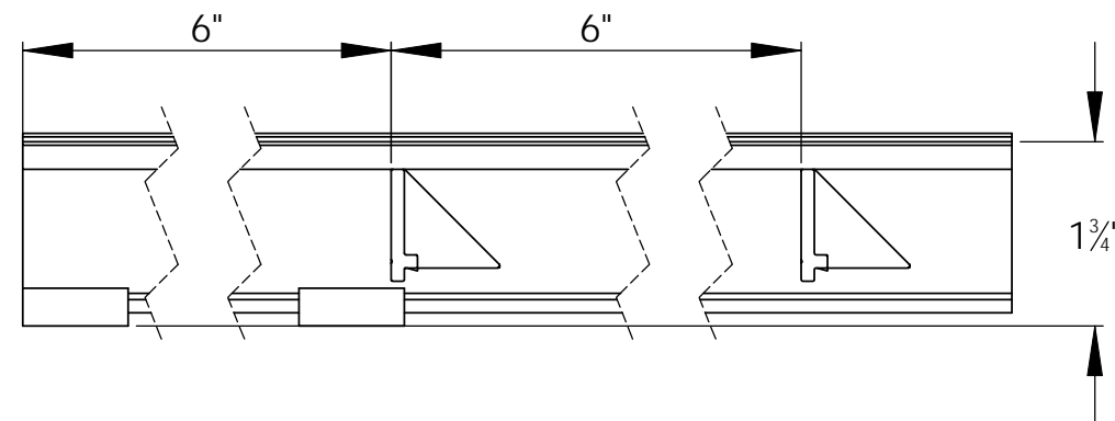
LENGTH VIEW
