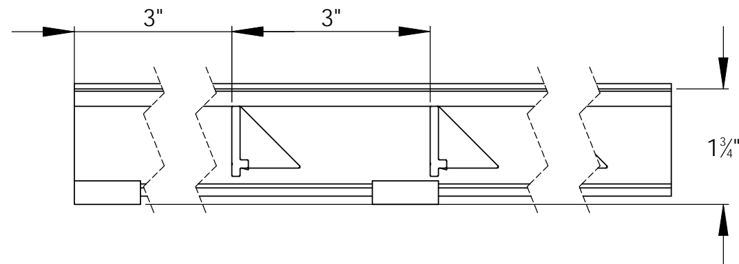
LENGTH VIEW
