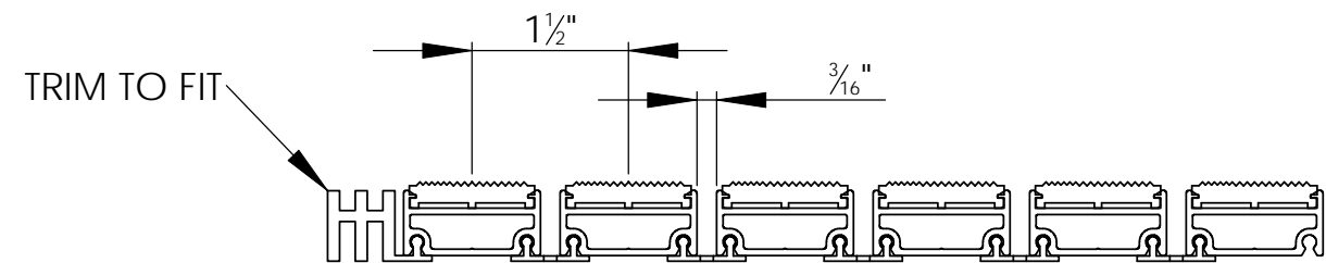
WIDTH VIEW
