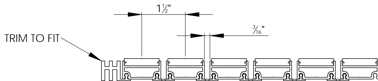
WIDTH VIEW
