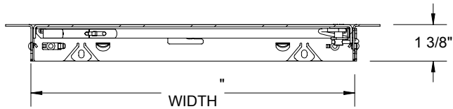
SECTION B-B
