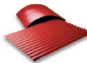
32" Coverage (813 mm) 2 3/4" (67 mm) 34 3/8" Coverage (880 mm)
