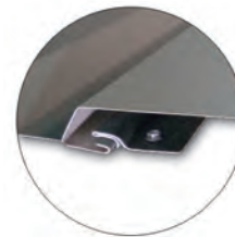
Detail of HS-12 & HS-8 Panel Interlock
