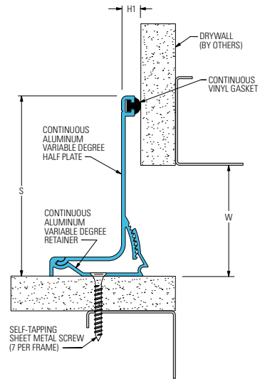
811-A09 Wall/Corner Wall/Ceiling (2" (50mm) system shown)
