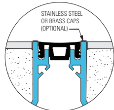
Decorative Caps (101-A01-025 system shown)
