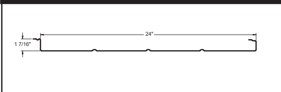
LP-15 Liner Panel
