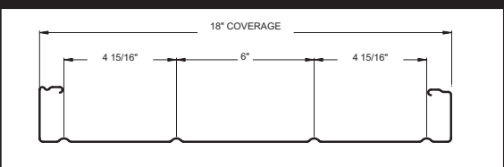
2 1/2" SSR
