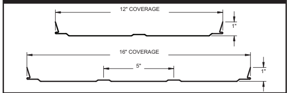
Grand Curve™
