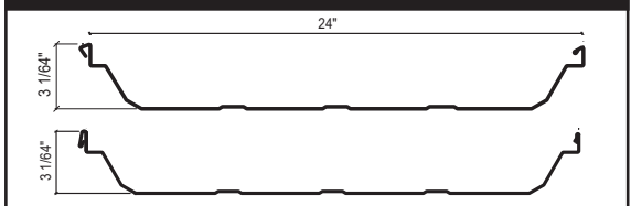
IP Seam 3 / IP Snap 3
