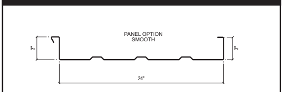
Seam Rib 324
