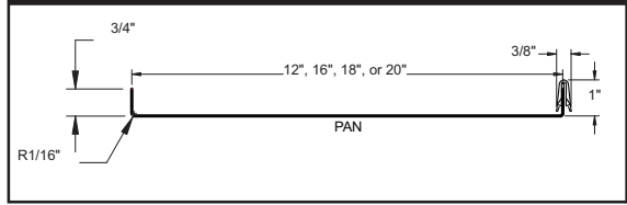
Snap-On-Seam
