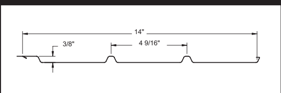
Posi-Lock Soffit
