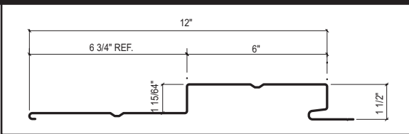
Select Series® 612 (612-R1 standard)
