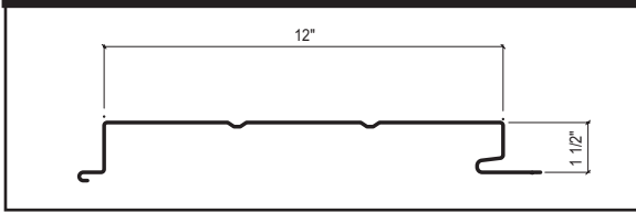
Select Series® 12 (12-R2 standard)
