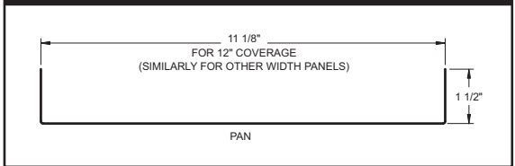
Snap-On-Batten
