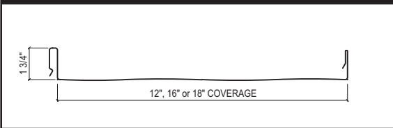
Thin Seam
