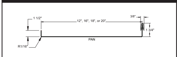
Snap-On-Seam High Profile
