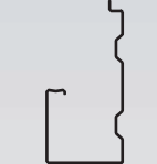
6" X 3" X .050 ROLLFORMED ALUMINUM FASCIA/GUTTER
