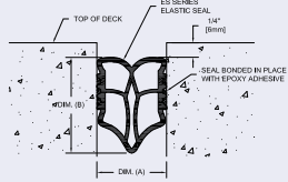
ES Elastic Seal (Relaxed Condition) *Other larger sizes available, call factory.
