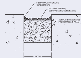
BCSW SERIES COMPRESSED WALL SEAL WITH COLORIZED SILICONE FACING 50% MOVEMENT AVAILABLE MAXIMUM LENGTH 42" (1067mm)
