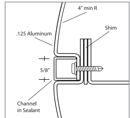
REVEAL JOINT
