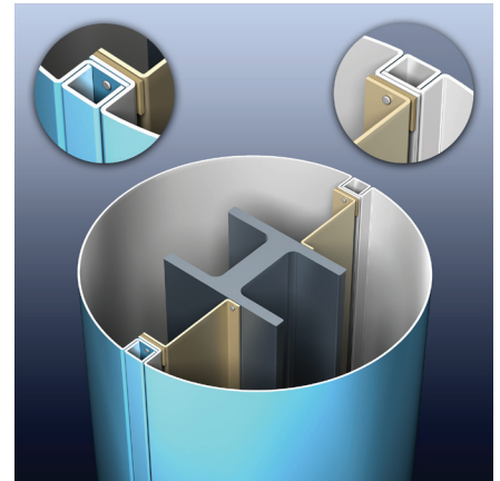
PAC 1000R
