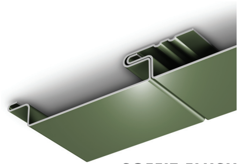
SOFFIT FLUSH
