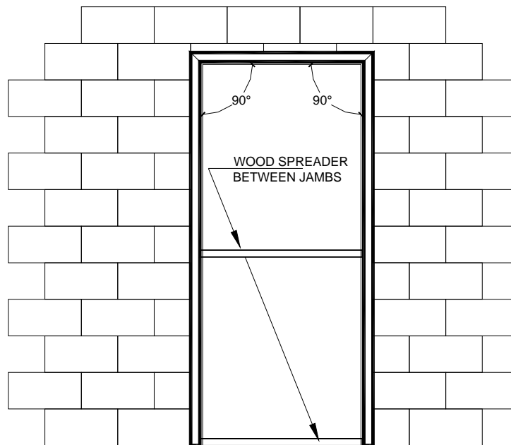
EXISTING MASONRY WALL CONSTRUCTION
