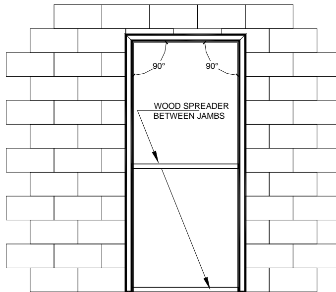
NEW MASONRY WALL CONSTRUCTION
