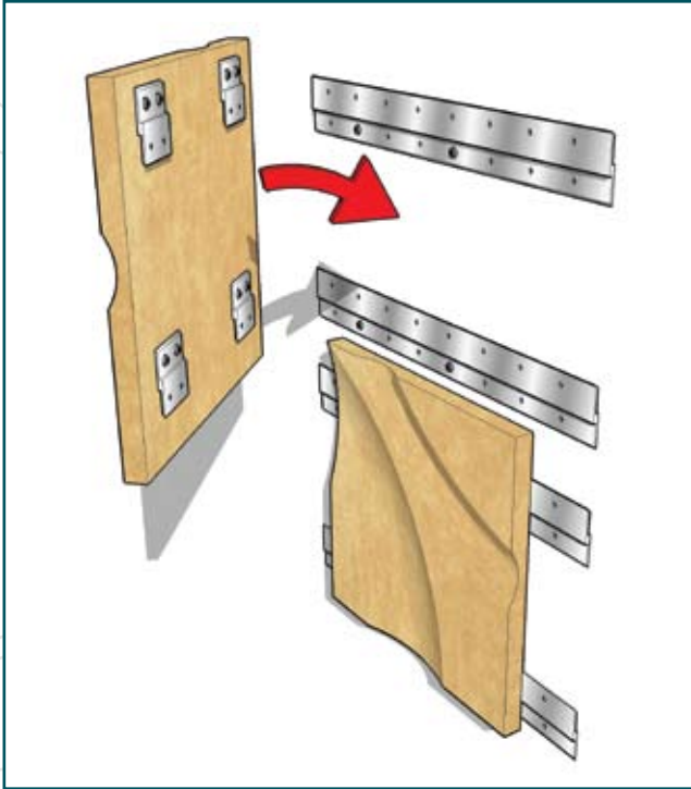
Proprietary wall rail hardware that holds panel assemblies is easily installed with simple tools
