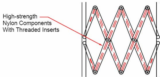
PLAN VIEW PANTOGRAPH CONTROL MECHANISM
