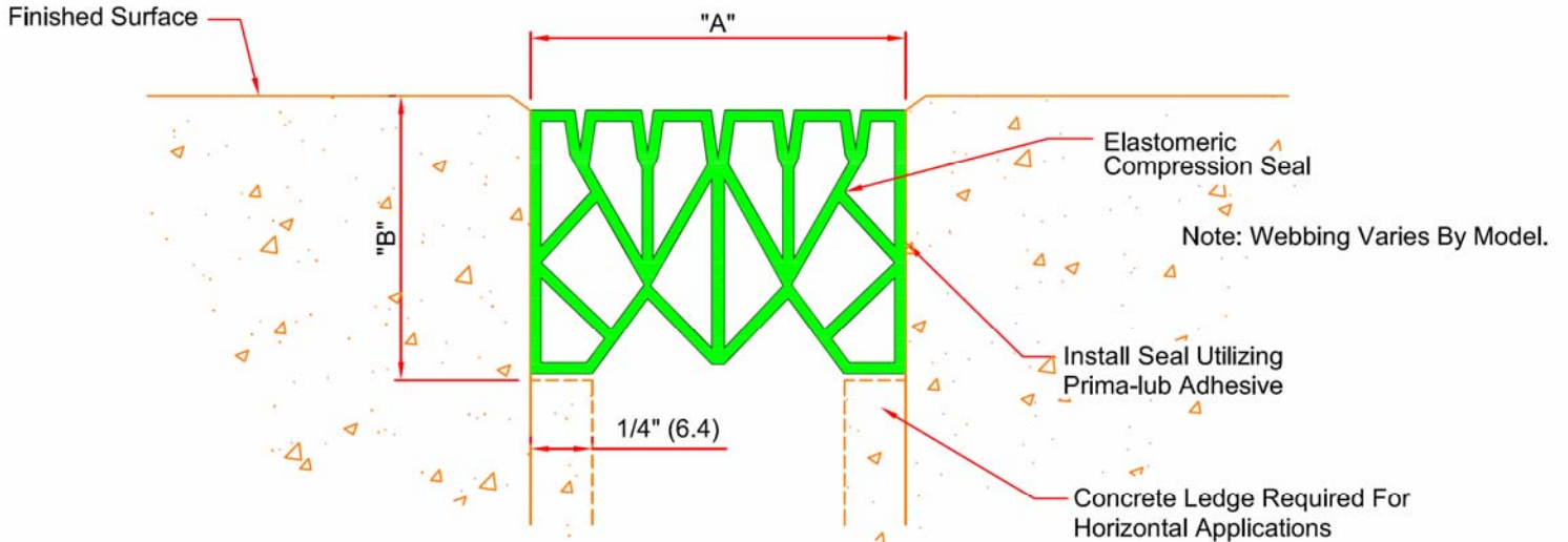
"EJ-SAN" PROFILE SLAB-TO-SLAB CONDITION
