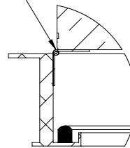
DETAIL E SCALE 1 : 3
