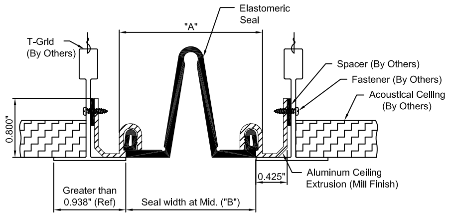
EJ-LCE DETAIL WITH SPACER CEILING TO CEILING CONDITION
