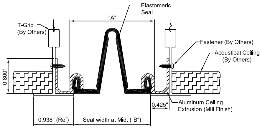
EJ-LCE STANDARD DETAIL CEILING TO CEILING CONDITION
