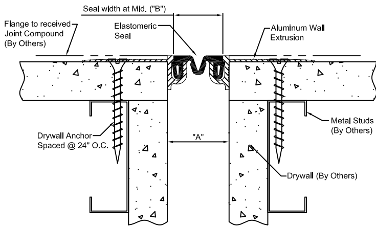
EJ-LCD-100 DETAIL WALL TO WALL CONDITION
