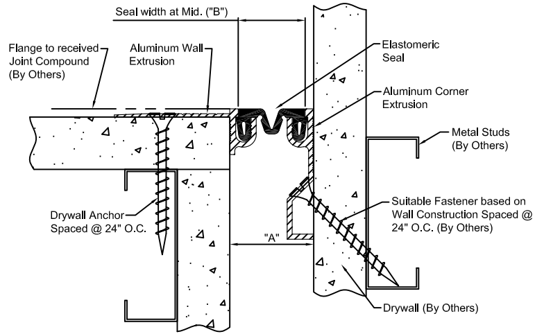
EJ-LCD-100W DETAIL WALL TO WALL CORNER CONDITION
