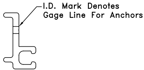
Aluminum Extrusion Part Number – 15003
