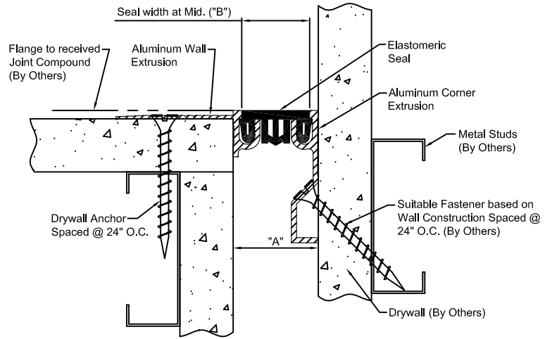
EJ-LCW-100W DETAIL WALL TO WALL CORNER CONDITION
