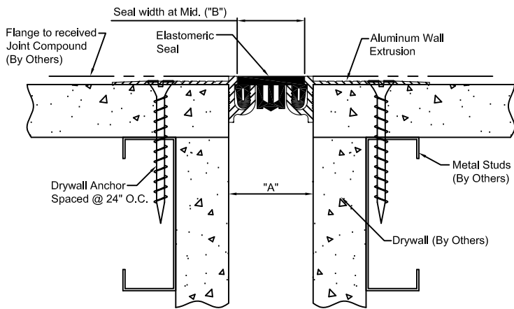
EJ-LCW-100 DETAIL WALL TO WALL CONDITION
