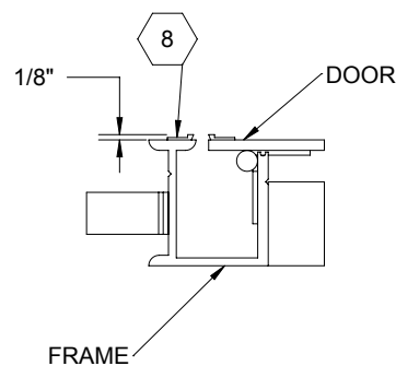
TILE EXTRUSION DETAIL
