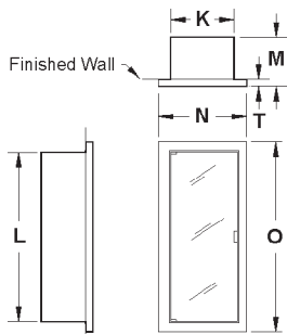
RECESSED
