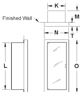
SEMI-RECESSED
