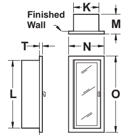
RECESSED
