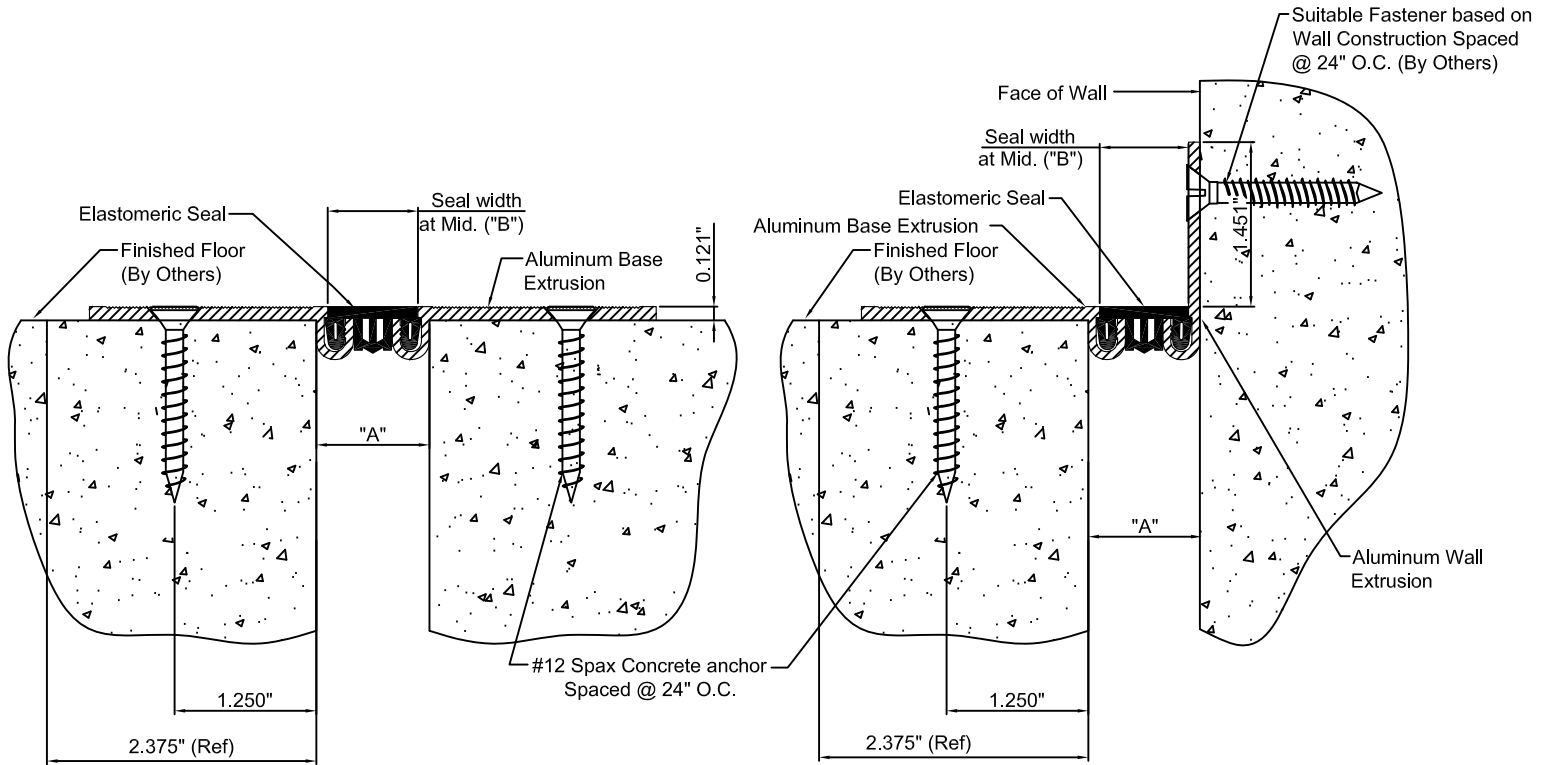
EJ-LCFT-100 DETAIL FLOOR TO FLOOR CONDITION
