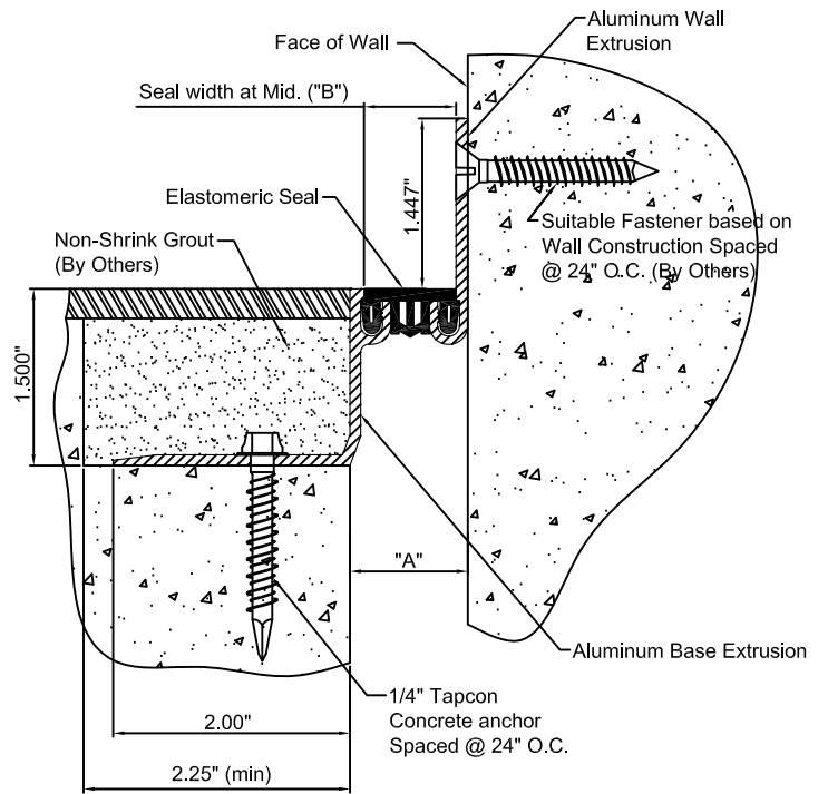
EJ-LCF-100W DETAIL FLOOR TO WALL CONDITION
