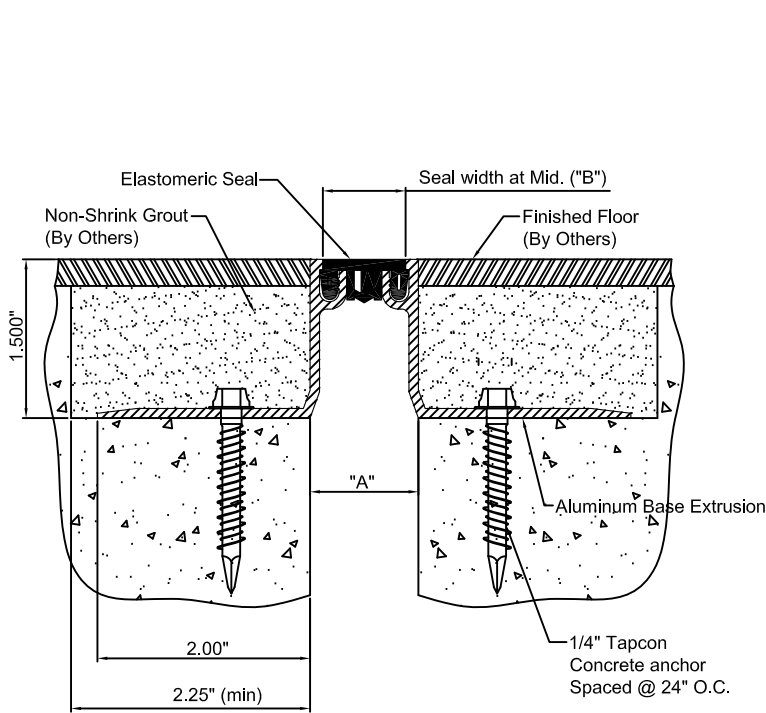
EJ-LCF-100 DETAIL FLOOR TO FLOOR CONDITION
