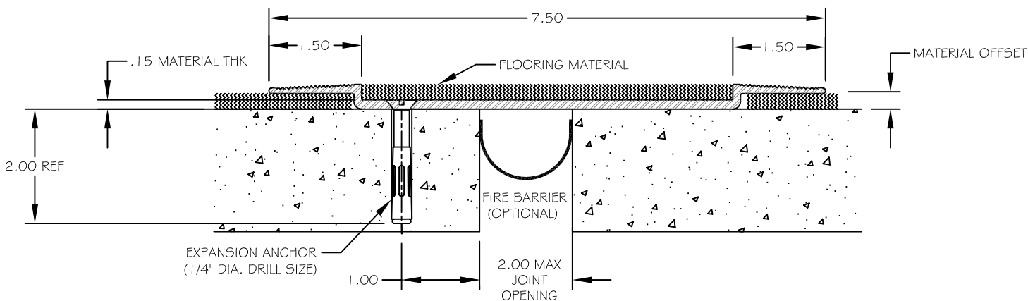
SURFACE CROSS SECTION (NOT TO SCALE)
