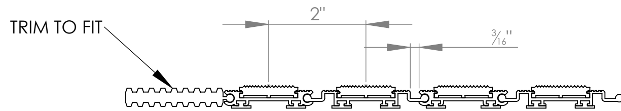
WIDTH VIEW
