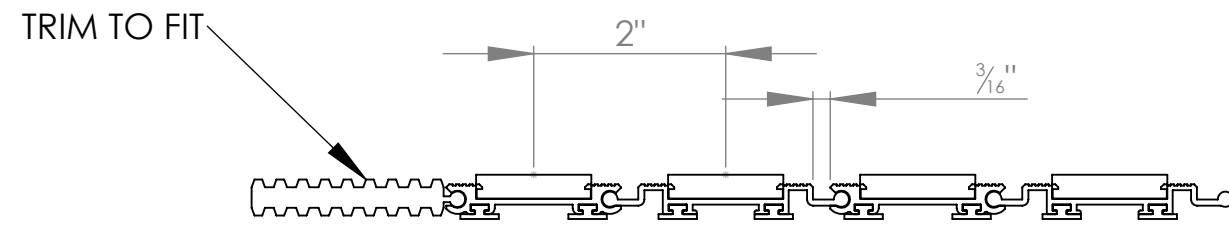
WIDTH VIEW
