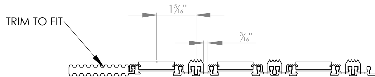
WIDTH VIEW
