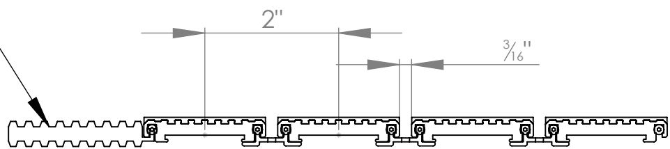
WIDTH VIEW
