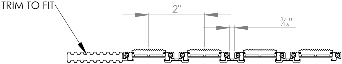
WIDTH VIEW
