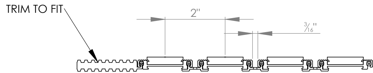
WIDTH VIEW
