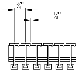
WIDTH VIEW
