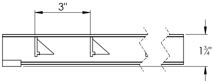
LENGTH VIEW
