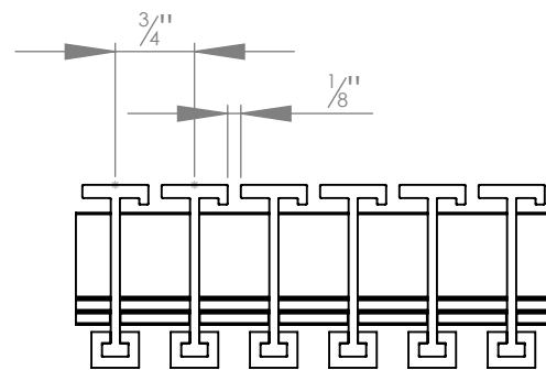
WIDTH VIEW
