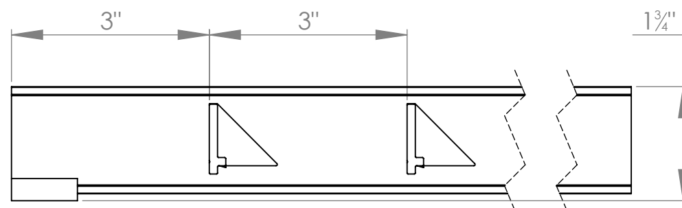
LENGTH VIEW
