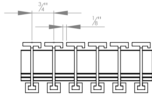
WIDTH VIEW
