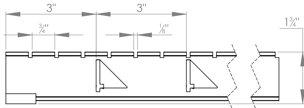
LENGTH VIEW
