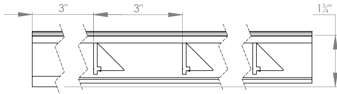
LENGTH VIEW
