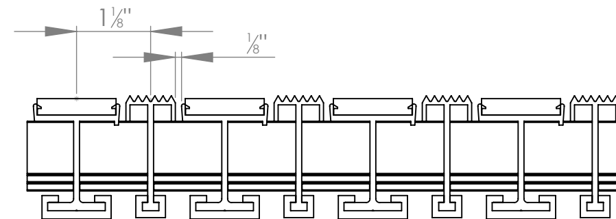
WIDTH VIEW
