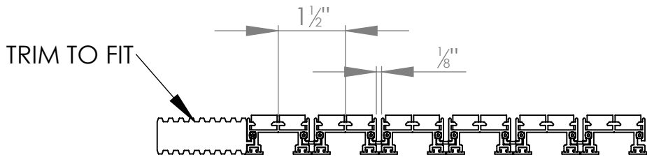
WIDTH VIEW
