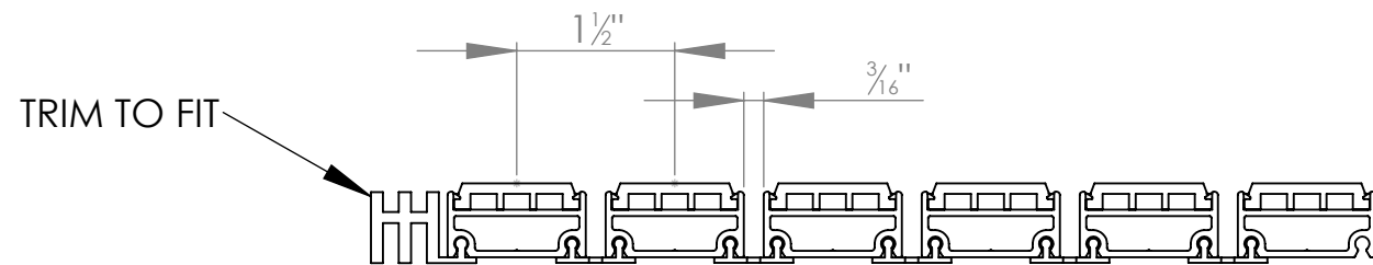
WIDTH VIEW
