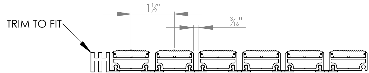
WIDTH VIEW
