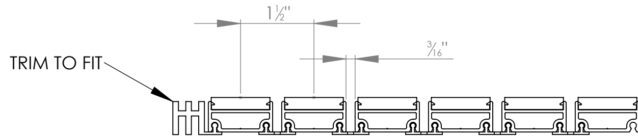
WIDTH VIEW
