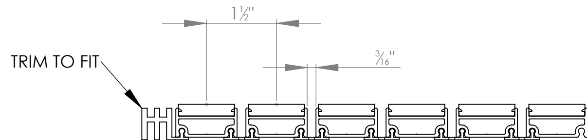
WIDTH VIEW
