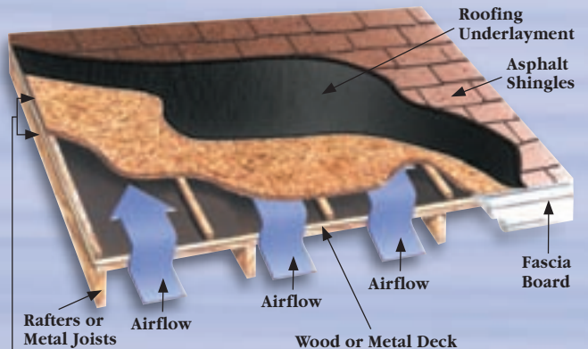
RMAX® VENTED NAILABLE BASE - 3
