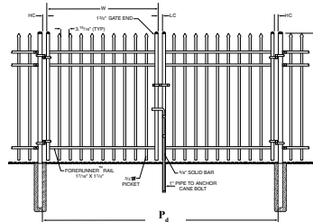
Order 2 Leaves For Double Swing Opening
