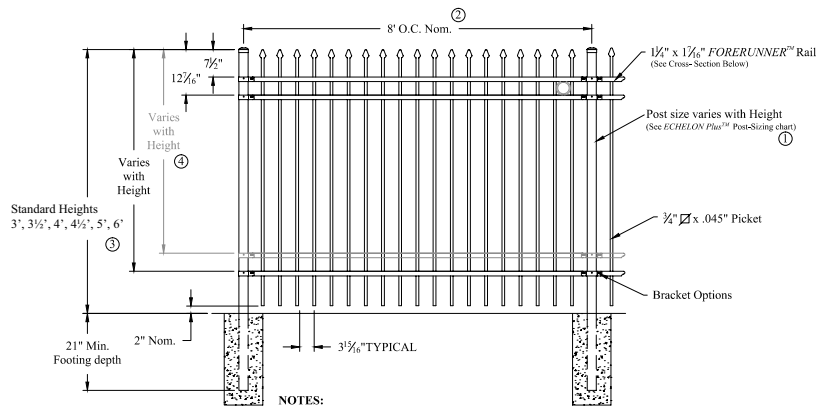
TYPICAL PANEL DRAWING (Classic Style shown; Majestic, Genesis, Warrior & Conqueror also available)
