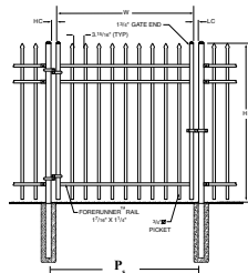
Order 1 Leaf For Single Swing Opening
