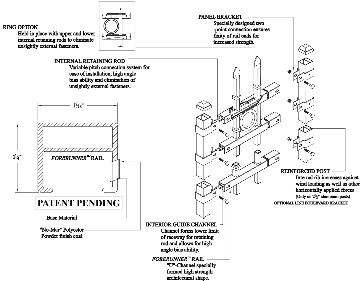
TYPICAL PANEL DRAWING (Classic Style shown; Majestic, Genesis, Warrior & Conqueror also available)
