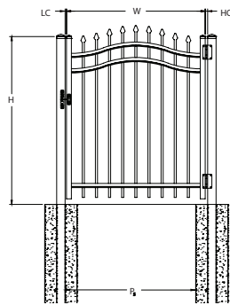
Order 1 Leaf For Single Swing Opening
