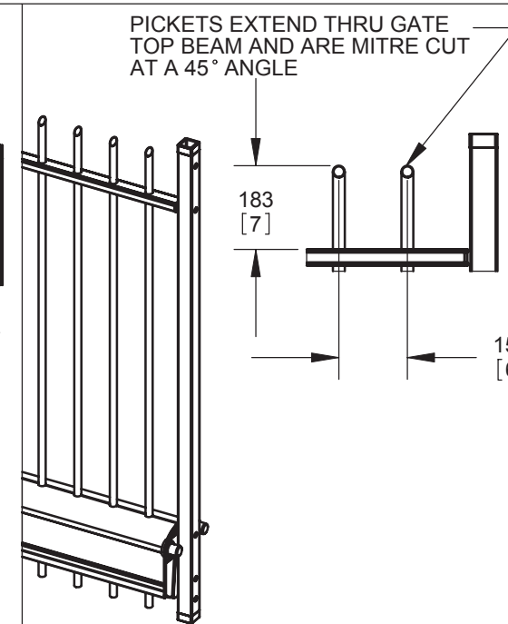
DETAIL 4-5B - ATLAS PANEL INFILL
