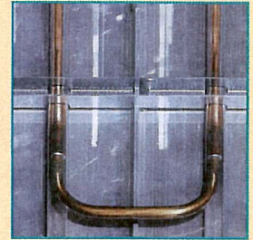
Low Pressure Drop Extruded Panel Back .578" ID Copper Tube
